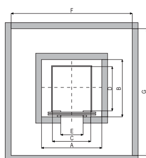
Hoistway Machine Room Plan For Auto Door
