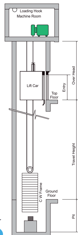
Hoistway Elevation Drawing
