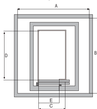
Hoistway Elevation Plan
