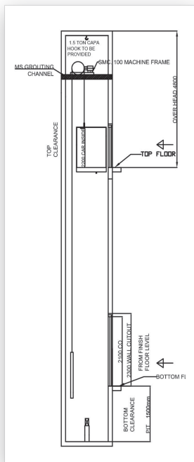
Hoist Way Machine Room Size Passenger Elevator with Manually Operated Doors
