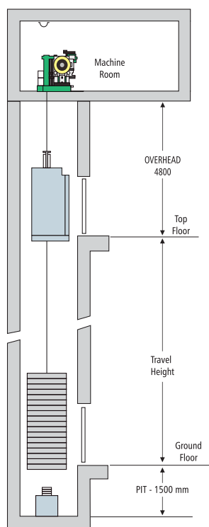
Hoistway Elevation Drawing
